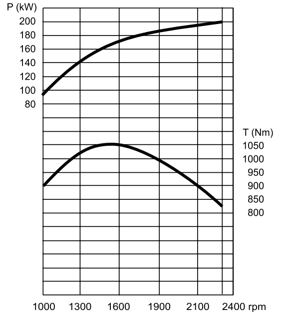
Engine TCD 2013 L6 2V
